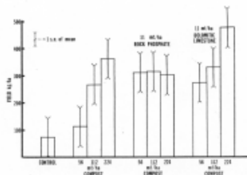
Figure 25-1. Forage yields (kg/ha) and birdfoot trefoil produced on an acid strip mine spoil amended with sewage sludge compost, rock phosphate, and dolomitic limestone
