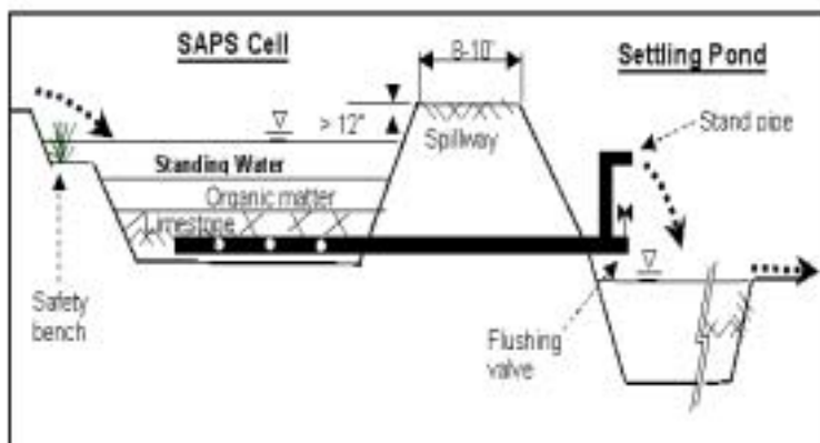
Figure 5. General Schematic of a SAPS Available at: http://sudan.cses.vt.edu/prp/Research_Results/SAPS.html
